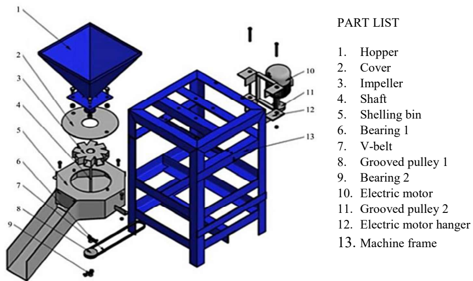
Figure 1. Exploded view showing structural components of a centrifugal cashew nut shelling machine by Kilanko et al. (2018)
